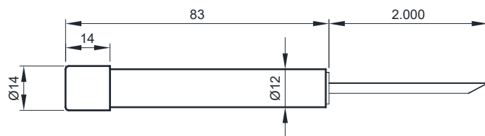
Dimension art. SM319017 and SM319018 (mm)
