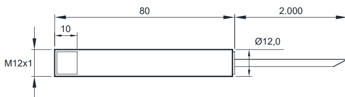
Dimension art. SM319016 (mm)
