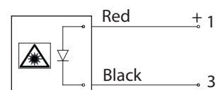
Cable connection
